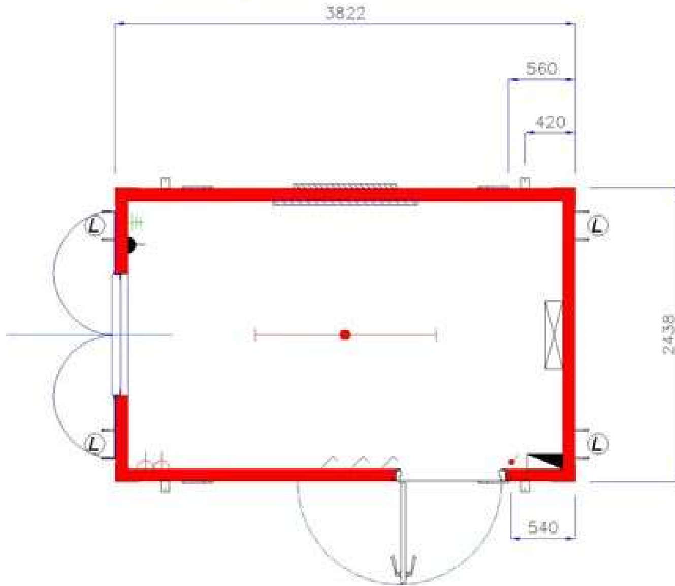
12x8' Open Plan Office
